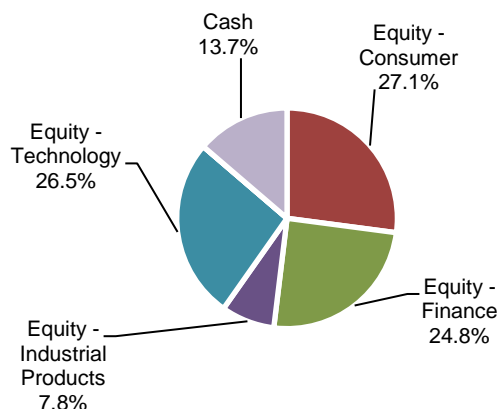
Asset & Sector Allocation of HLDGF as at 30 June 2022
